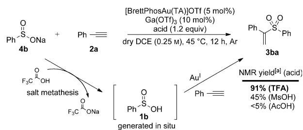
Scheme 2. One-pot synthesis of vinyl sulfone 3ba from bench-stable sodium benzenesulfonate ( 4b ). [a] Yield determined by 1 H NMR spectroscopy with 1,3,5-trimethoxybenzene as the internal standard.
