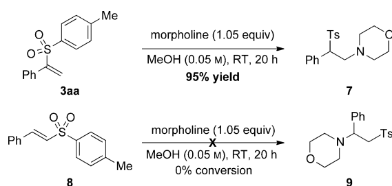
Scheme 4. Comparison of the aza-Michael addition of morpholine to \alpha - or \beta -substituted vinyl sulfones. Ts = 4-toluenesulfonyl.
