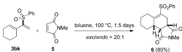
Scheme 3. Diels-Alder reaction between 2-sulfonyl diene 3bk and N-methyl maleimide ( 5 ).
